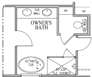
OPT. OWNER'S BATH 1 FLOOR PLAN
