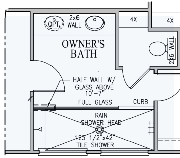
OPT. OWNER'S BATH 2 FLOOR PLAN
