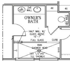
OPT. OWNER'S BATH 2 FLOOR PLAN
