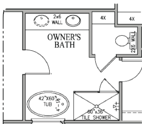
OPT. OWNER'S BATH 1 FLOOR PLAN
