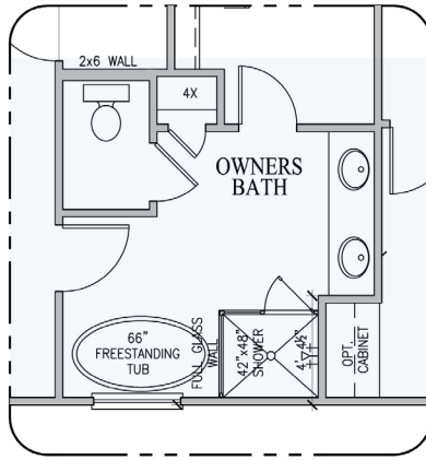
OPT. OWNERS BATH 2 FIRST FLOOR PLAN
