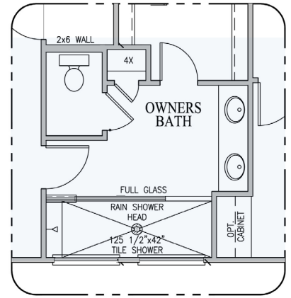
OPT. OWNERS BATH 3 FIRST FLOOR PLAN
