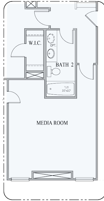
OPT. MEDIA ROOM SECOND FLOOR PLAN
