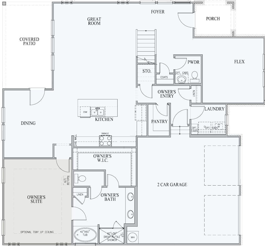
FIRST FLOOR PLAN - TRADITIONAL 1
