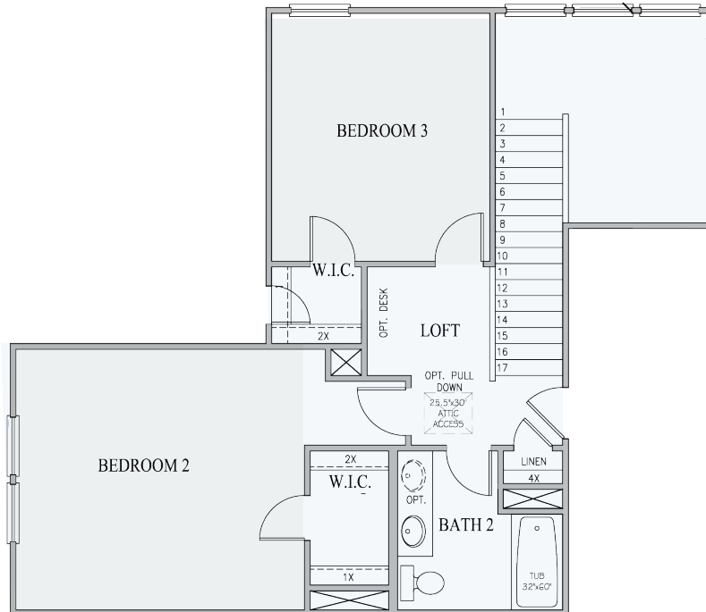
SECOND FLOOR PLAN - TRADITIONAL 1
