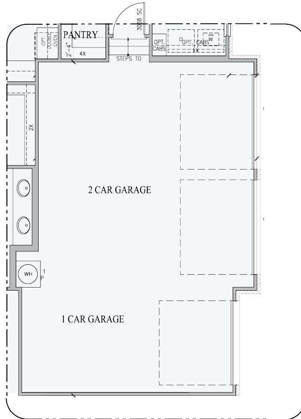
OPT. 3 CAR FRONT LOAD FIRST FLOOR PLAN
