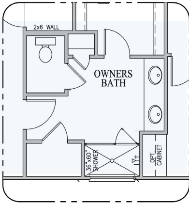
OPT. OWNERS BATH 1 FIRST FLOOR PLAN
