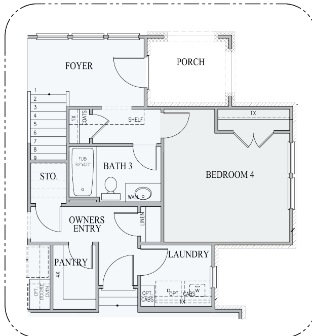
OPT. BEDROOM 4 FIRST FLOOR PLAN
